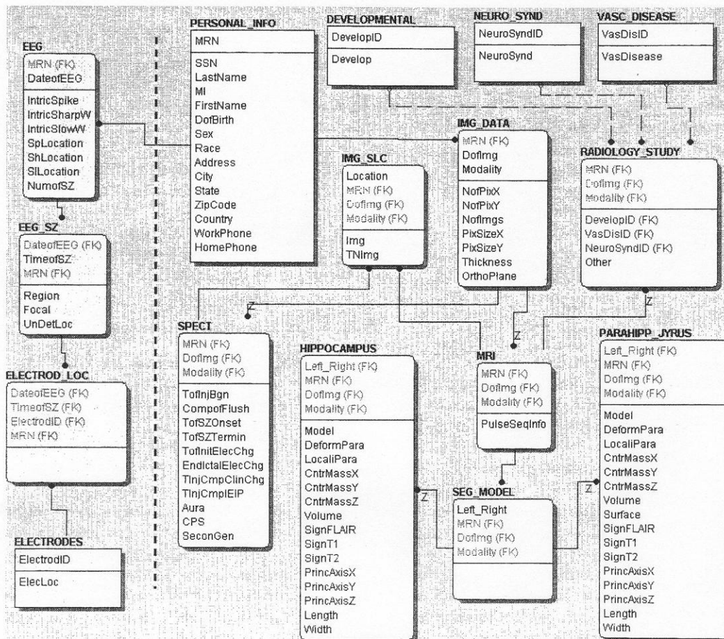
Figure 6: The conceptual sub-schema diagram for inpatient EEG study (left portion of the dashed line), and image studies (only the key attributes and relationships are shown).
